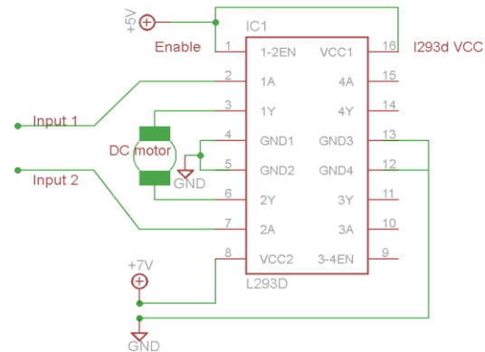
Fig 3 L293D Motor Driver IC ARDUINO
