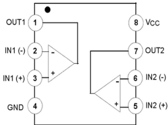
Fig 5 LM358 IC Pin Diagram DC GEAR MOTOR
