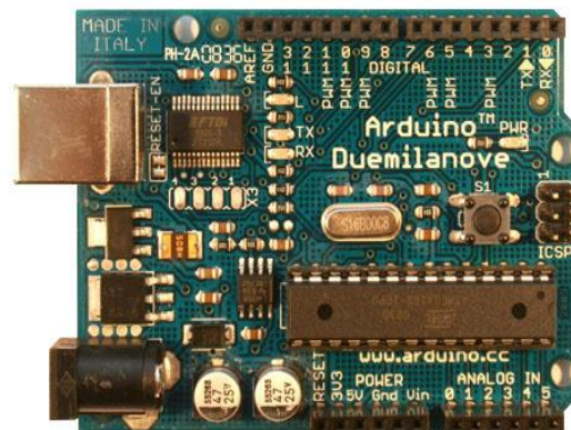
Fig 4 Arduino Board LM358 IC
